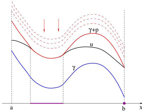
Figure 1: An example of a solution to the obstacle problem (3.3)-(3.4). Note that u_x(a) = 0 but at the point b one has u(b) = \gamma(b) + p and \gamma_x(b) < u_x(b) < 0 . If the measure \mu concentrates a positive mass on the boundary \partial\Omega , solutions to the variational inequality (3.6) need not satisfy the boundary condition (1.2) in the classical sense. Theorem 3.3 is proved by solving the obstacle problem (3.6) with various choices of p \geq 0 , and finding a value of p for which (3.1)-(3.2) hold.
