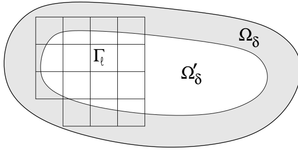
Figure 2: The decomposition of the domain \Omega = \Omega_\delta \cup \Omega'_\delta , where the inner domain is covered by finitely many hypercubes \Gamma_\ell .
