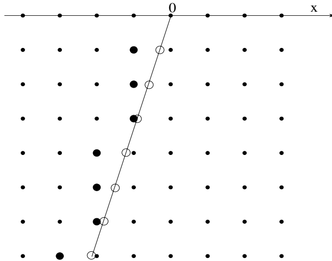
FIGURE 2.1. Discrete sources at integer points.
