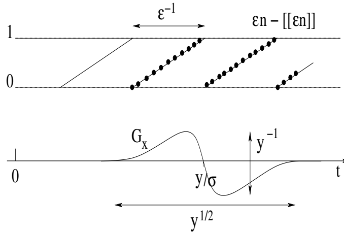
FIGURE 2.2. Interaction of G_x and fractional parts.
