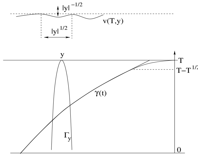
FIGURE 2.3. Oscillations produced by sources along the curve \gamma(t) .
