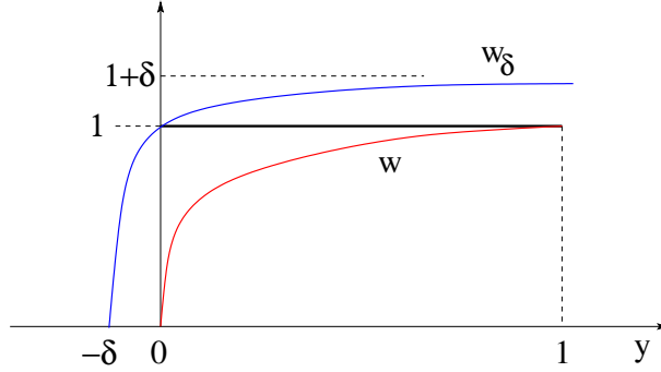
Figure 6: The function w at (6.32), used to construct a lower solution to (6.42), and the functions w_\delta at (6.34)-(6.35), used to construct upper solutions.
