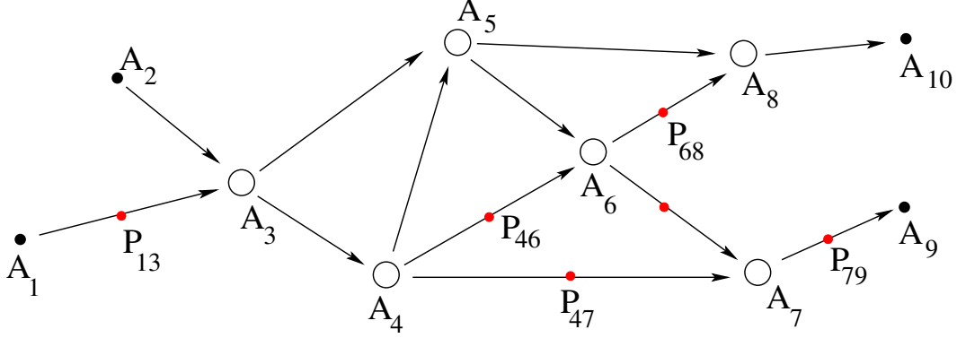
Figure 3: In this network, A_1, A_2 are entrance nodes, A_3, \dots, A_8 are transit nodes, and A_9, A_{10} are exit nodes. We denote by P_{ij} the mid-point of the arc \gamma_{ij} from A_i to A_j . f:tf143
