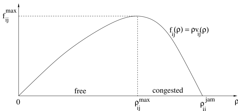
Figure 1: The flux f_{ij} as a function of the density \rho , along the arc \gamma_{ij} from the node A_i to A_j . f:tf142
