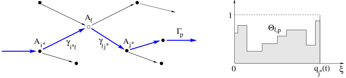
Figure 4: Left: a node A_\ell along the path \Gamma_p . Right: the function \xi \mapsto \Theta_{\ell,p}(t, \xi) , determining the distribution of p -drivers within the queue q_{j^*} . f:tf200
