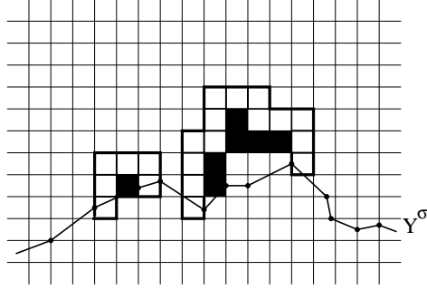
Figure 6: Two j -black islands and the surrounding paths of j -white squares, providing the detours.
