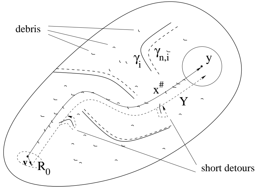
Figure 3: Constructing a trajectory x_n(\cdot) which reaches a point close to y , avoiding the walls in \gamma_n .
