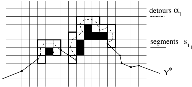
Figure 8: The curve Y^* . Compared with Y^\sigma in Figure 6, some segments s_i have been removed and replaced by the detours \alpha_\ell , to get around black islands.
