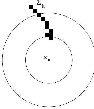
Figure 7: A chain of black squares joining a point in B(x, r) to a point outside B(x, 2r) must contain at least r/\sqrt{2}\sigma_k squares.
