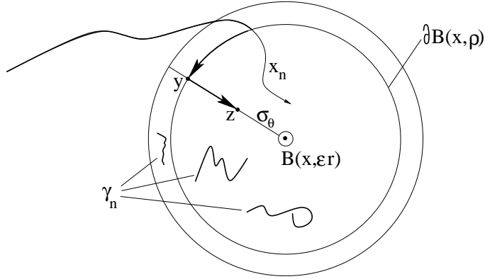
Figure 10: The trajectory x_n^\sharp , reaching z and avoiding the walls \gamma_n .
