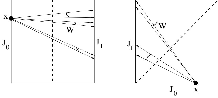
Figure 1: The projections \pi_x(W) and \pi_x(W \cap T_x) : on the left the case where J_0 and J_1 are opposite sides, on the right the case where they have a vertex in common.
