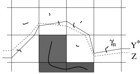
Figure 9: The curve Y^* (solid line) and a \mu -close polygonal Z which avoids the walls in \gamma_n .
