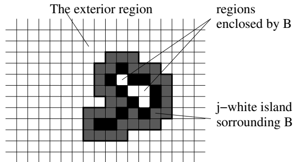
Figure 5: A j -black island B , the regions enclosed by the island, the exterior region and the j -white island surrounding B .
