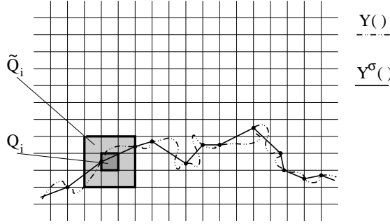
Figure 4: The grid of mesh \sigma and the new trajectory Y^\sigma
