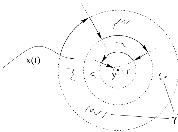
Figure 2: Constructing an admissible trajectory that reaches the point y avoiding the wall \gamma .
