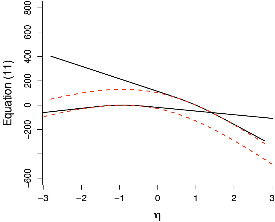
Figure 2: For a simplistic model with g(\mathbf{y}) equal to the number of edges, the dotted curves show \ell(\theta) - \ell(\theta_0) for two different values of \theta_0 , namely \theta_0 = 1 (upper curve) and \theta_0 = -1 (lower curve). The solid curves are the corresponding approximations using equation (11). The true MLE, \hat{\theta} = -0.9072 , is easily derived in this case. Note that \theta_0 = -1 appears to give a good approximation to the loglikelihood near \hat{\theta} , whereas \theta_0 = 1 gives an approximation that cannot even be maximized.
